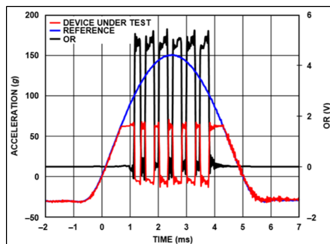
Figure 2: Signal behavior under overload (source: Analog Devices)
